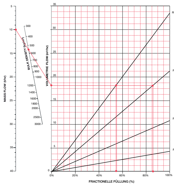
Capacity Chart
